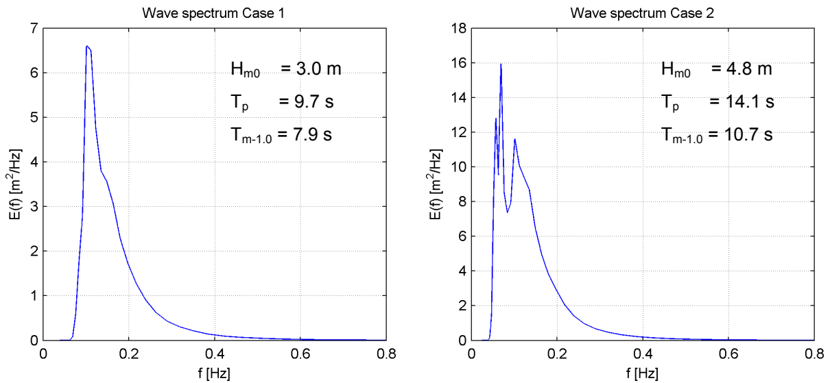
Figure 2: Imposed wave spectra for case C1 (left) and C2 (right).
